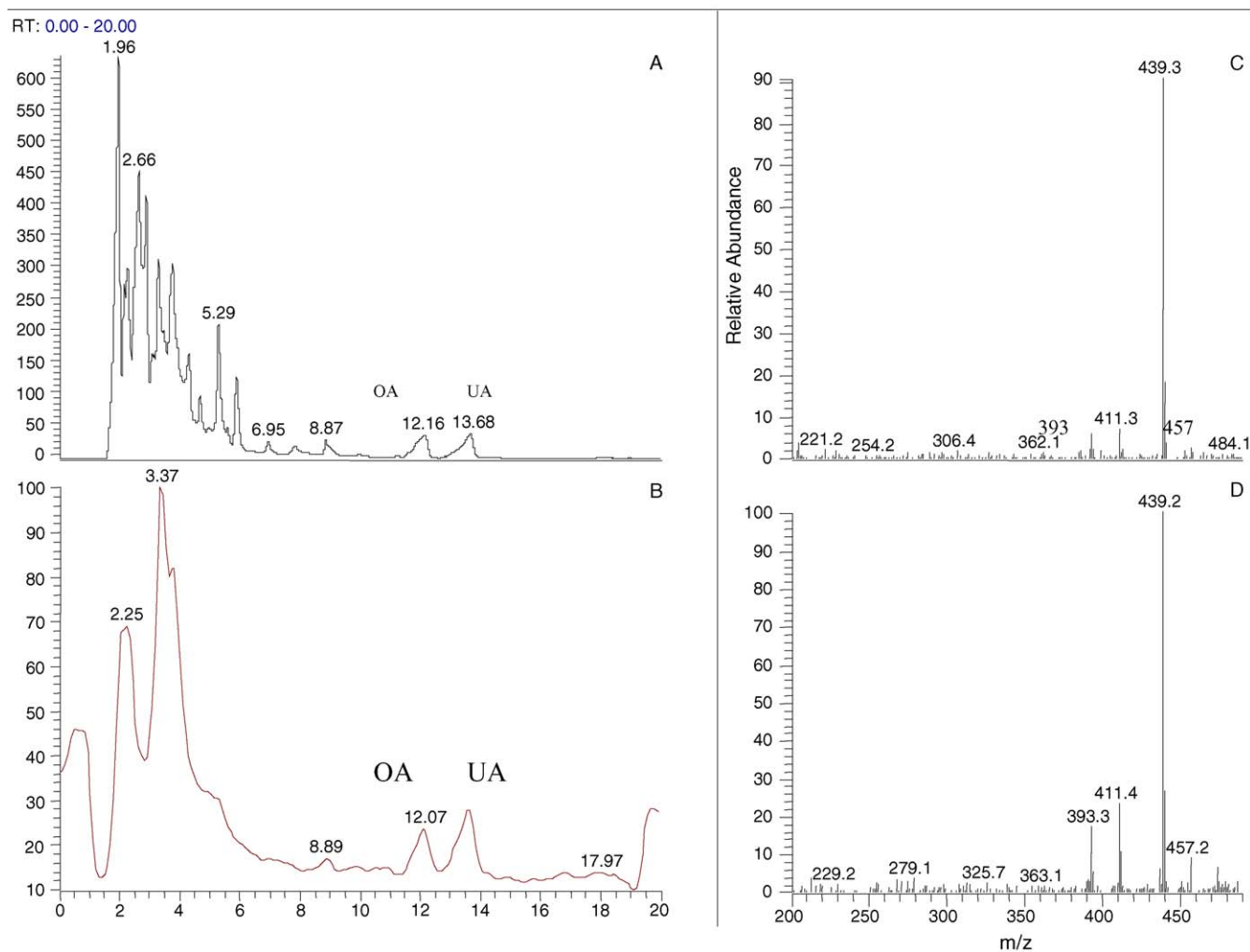
Fig. 2. LC/UV (215 nm: A) and LC/MS (TIC: B) chromatograms of the plant dichloromethane extract and full MS spectra ( m/z 200–490) of OA (C) and UA (D) peaks.
